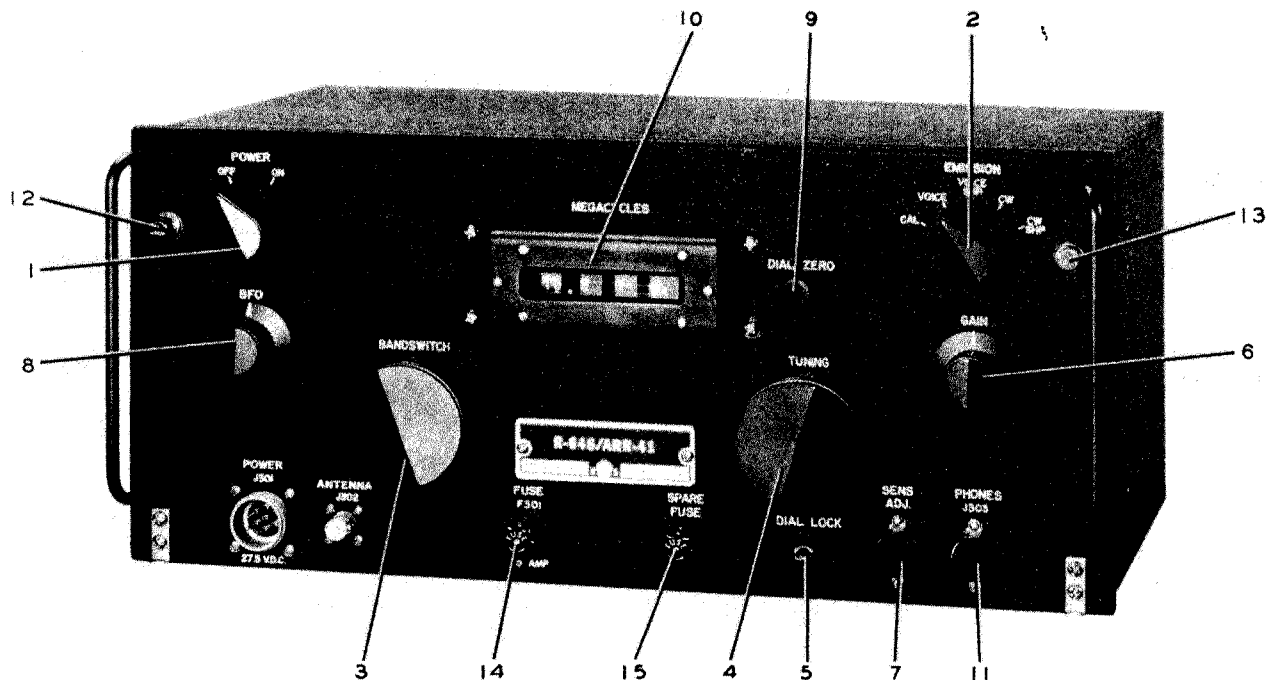
Figure 2-1. Radio Receiver R-648/ARR-41, Front Panel Controls
